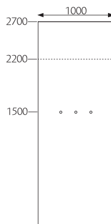
Coat hooks Ø32 x 45 mm
