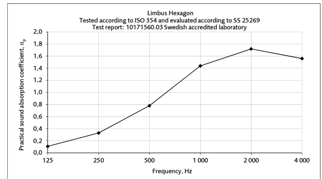
Ekvivalent absorptionsyta per m 2 skärmyta (m 2 S/m 2 )
