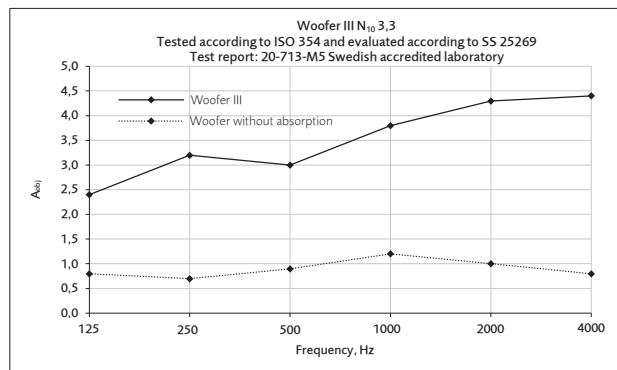
Sound absorption area according to ISO 354 and SS 25269
