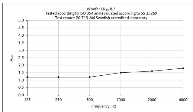
Sound absorption area according to ISO 354 and SS 25269
